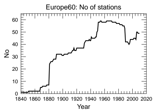
Figure A.21: The variation in numbers of stations in the Europe60 average
