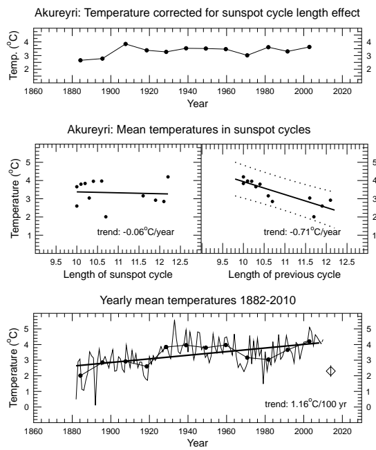
Figure 16: Akureyri, Iceland, average yearly temperatures, explanation as in figure 4.
