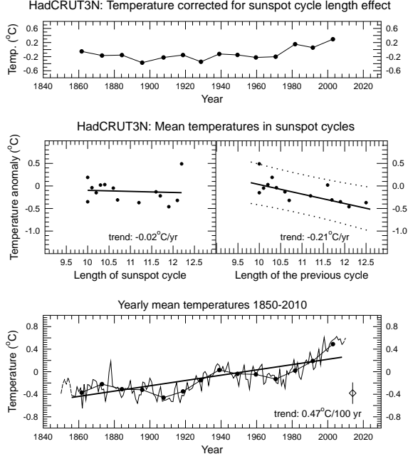
Figure 19: HadCRUT3N, average yearly temperature anomalies, explanation as in figure 4.
