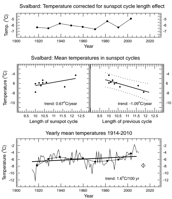
Figure 17: Svalbard (Longyearbyen), average yearly temperatures, explanation as in figure 4.
