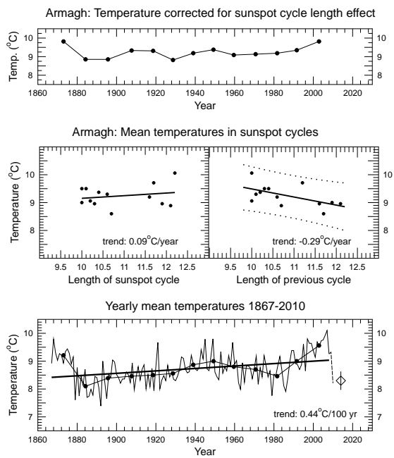
Figure 14: Armagh, Northern Ireland, average yearly temperatures, explanation as in figure 4.
