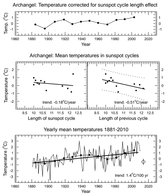
Figure 13: Archangel, Russia, average yearly temperatures, explanation as in figure 4.
