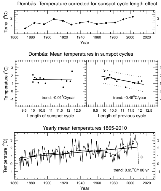
Figure 5: Dombås, Norway (Inland, mountain valley 62N), explanation as in figure 4
