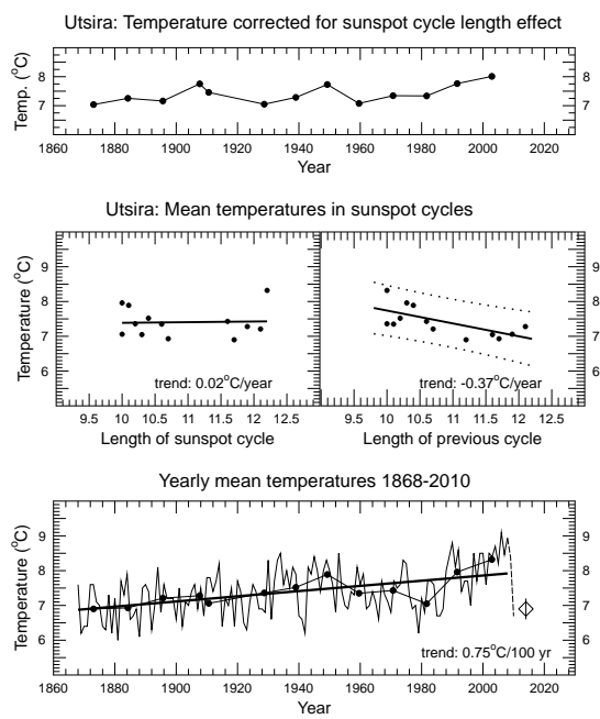
Figure 9: Utsira lighthouse, Norway, average yearly temperatures, explanation as in figure 4.
