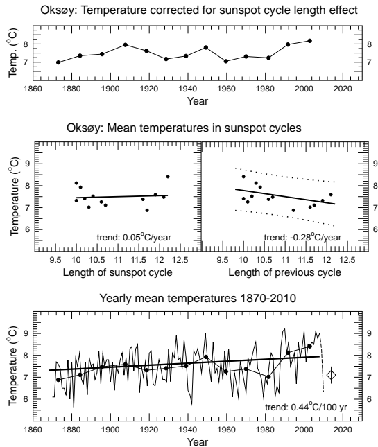
Figure 8: Oksøy lighthouse, Norway, average yearly temperatures, explanation as in figure 4. The confidence interval indicated in the center right panel is probably less than 95% in this case.
