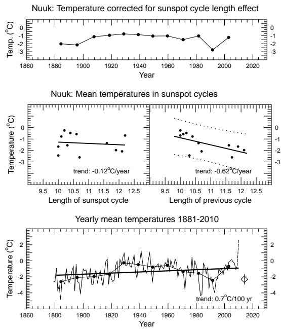
Figure 18: Nuuk, Greenland, average yearly temperatures, explanation as in figure 4.
