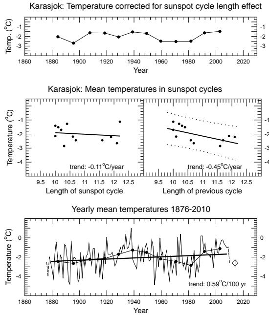
Figure 11: Karasjok, Norway, average yearly temperatures, explanation as in figure 4.
