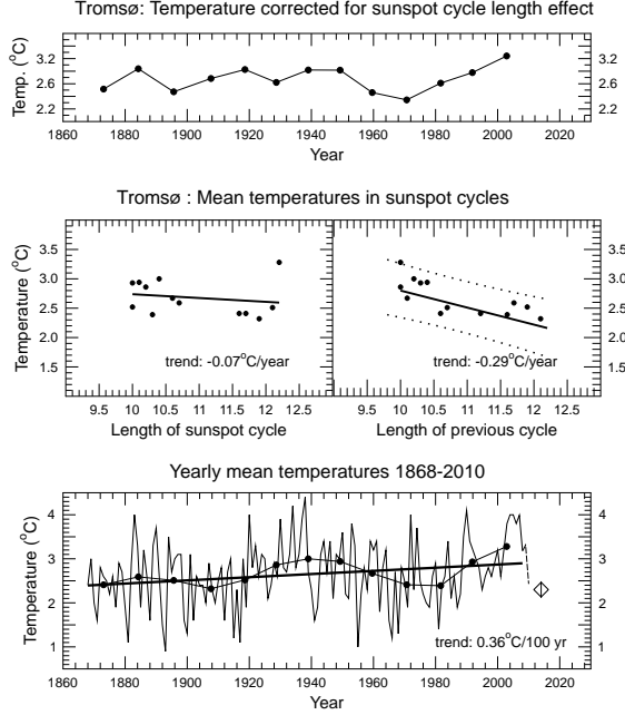
Figure 4: Tromsø, Norway (Coastal city 70N): Lower panel: Annual mean temperatures and mean temperatures in sunspot cycles (dots) with linear trend. The broken line shows temperatures measured so far in SC24. The center two panels show temperatures in sunspot cycles versus SCL (left) or PSCL (right). In the right center panel the 95% confidence interval is indicated with dotted lines. The lower panel shows the forecasted value for SC24 (diamond) with standard deviation error bar. The top panel shows the residuals from the t(PSCL) model, and represents what may be left for other regressors and noise to explain.
