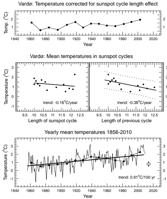
Figure 12: Vardø, Norway, average yearly temperatures, explanation as in figure 4.
