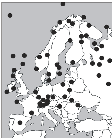
Figure A.20: The location of the Europe60 stations
