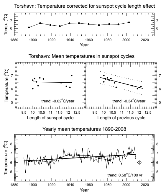
Figure 15: Torshavn, Faroe Islands, average yearly temperatures, explanation as in figure 4.
