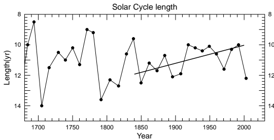
Figure 1: Length of solar cycles (inverted) 1700-2009. The last point refers to SC23 which is 12.2 years long. The gradual decrease in solar cycle length 1850-2000 is indicated with a straight line.
