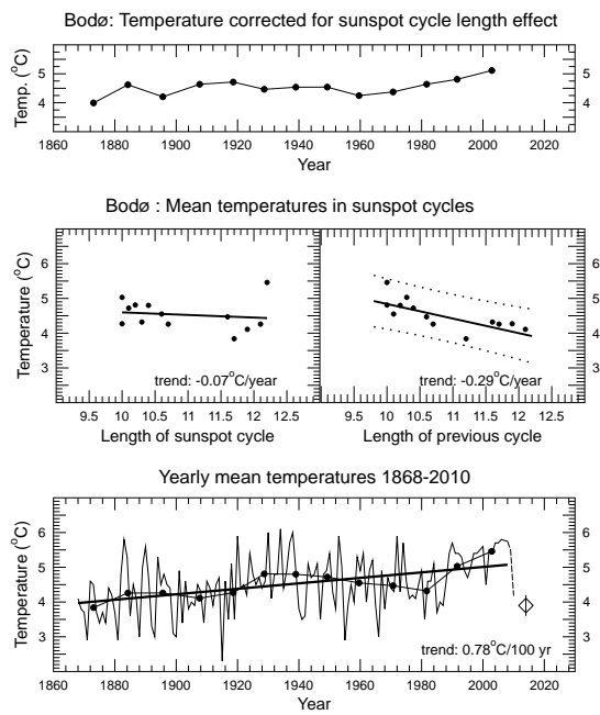
Figure 10: Bodø, Norway, average yearly temperatures, explanation as in figure 4.
