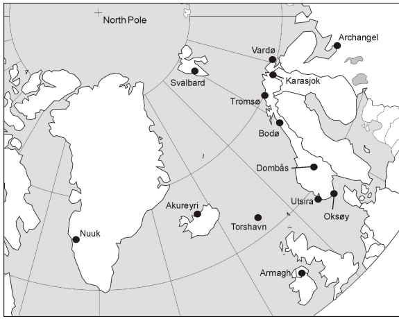
Figure 2: The location of meteorological stations with temperature series analyzed.
