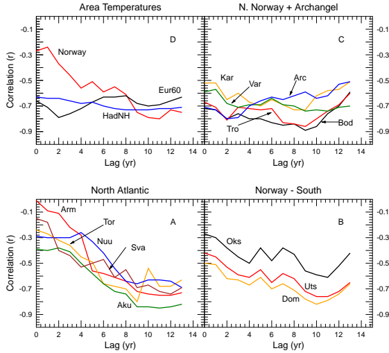
Figure 3: Correlations between SCL and 11 years average temperatures as function of time lag after the mid time of the sunspot cycle.
