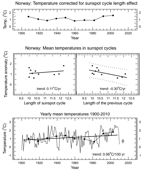
Figure 6: Norway, average yearly temperatures, explanation as in figure 4.
