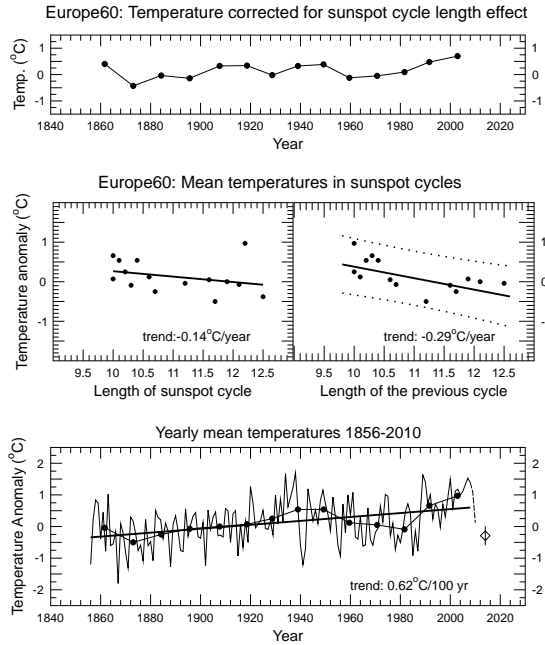
Figure 7: Temperature anomaly for 60 stations on land in Europe, mostly located outside large cities. A list of the stations is given in the Appendix, explanation as in figure 4.
