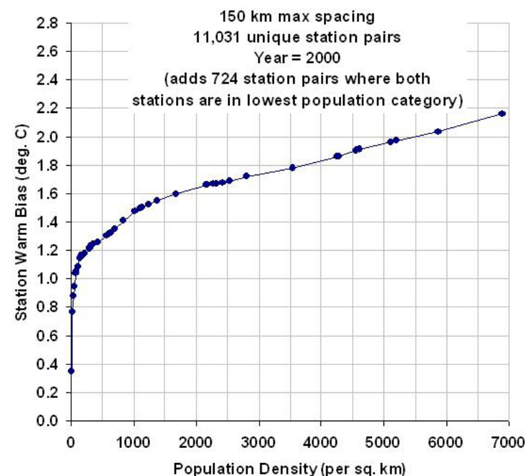
Fig. 4. Localized warming (Urban Heat Island effect) at temperature monitoring stations occurs as population density increases, as seen in this analysis of one year of daily temperature data from all reporting stations in the world. Note the most rapid warming occurs at the lowest population densities.
