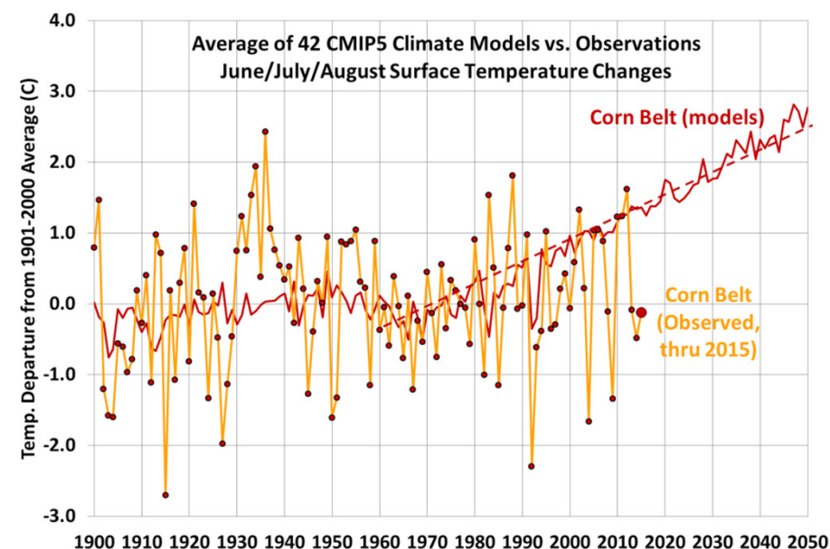
Fig. 10. Comparison of the average surface temperature predictions across 42 climate models versus observations for the primary U.S. Corn Belt states (IA, IL, IN, KS, MI, MN, MO, NE, ND, OH, SD, WI) also shows the models are warming faster than the real climate system (official NOAA data).
