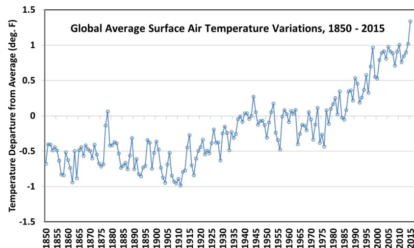
Fig. 8. Surface-based thermometer estimates of global average temperature, after adjustments, show about a 1.5 F temperature increase over the last 150 years (HadCRUT4 data).
