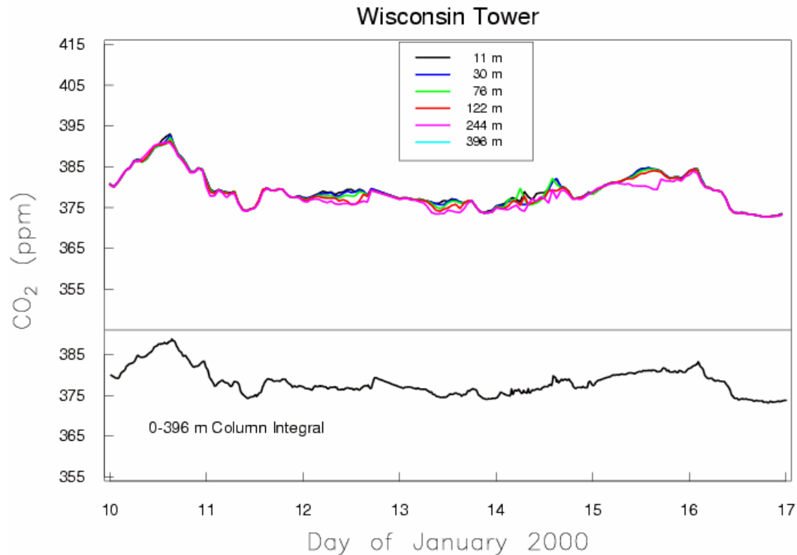
Figure 26. Measurements of CO 2 concentrations for a week in January 2000, Wisconsin Tower
