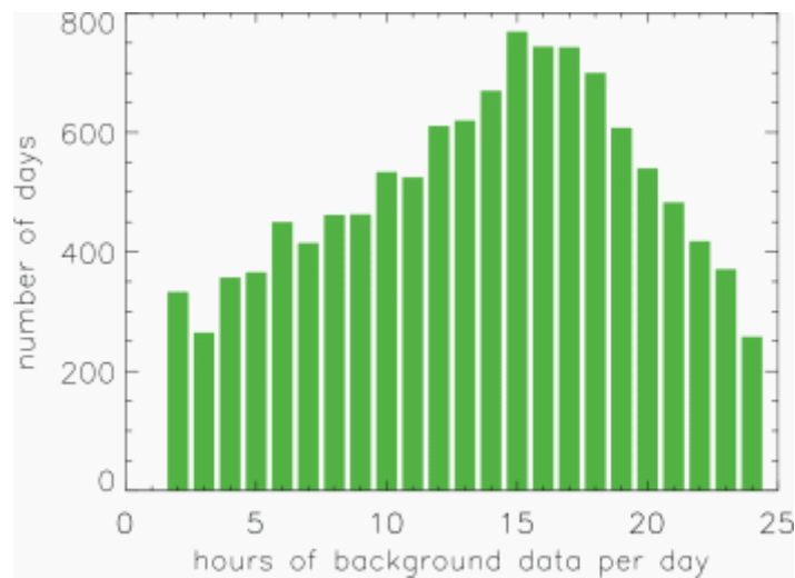
Figure 20. Distribution of number of hourly data retained
