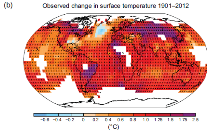
Figure 3: Observed change in surface temperature 1901–2012 [p. 6]
