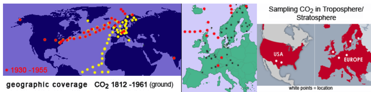
Figure 29. Distribution of chemical measurements
