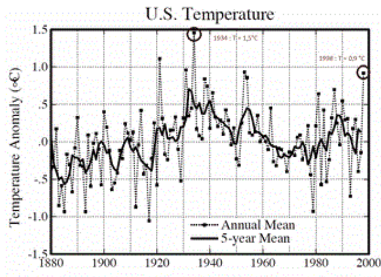
Figure 7. Annual mean and five-year mean temperature anomalies for 48 US states, in relation to the reference period 1951-1980 (1999 version)
