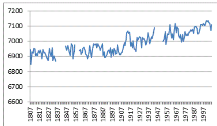
Figure 42: Ocean level records for Brest since 1807 (SHOM)
