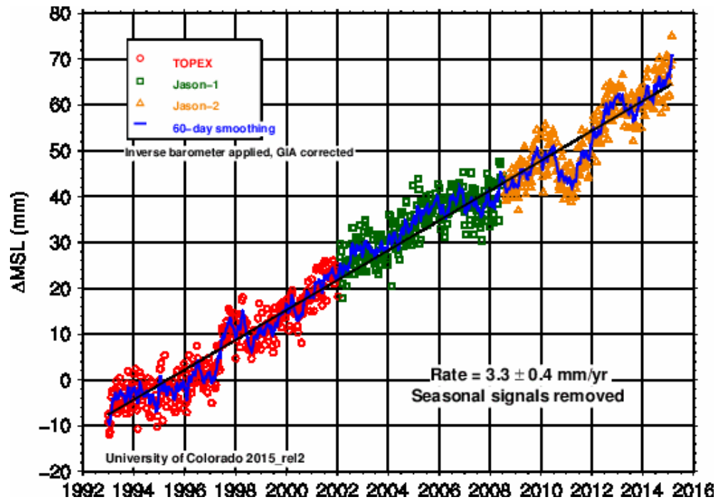
Figure 37: Changing sea levels over time
