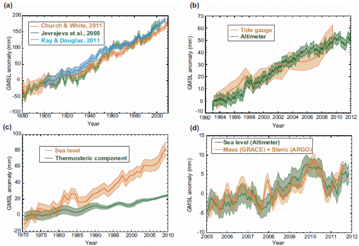
Figure 5: Sea level according to different techniques, 1970–2010
