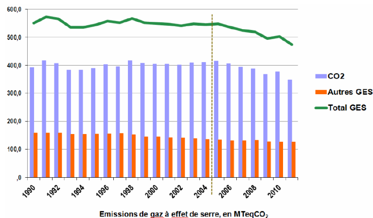
Figure 1: France's GHG emissions [French Audit Office]
