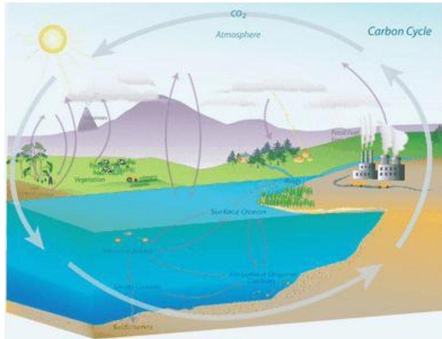
Figure 14. The carbon cycle (source: Barb Deluisi, NOAA)
