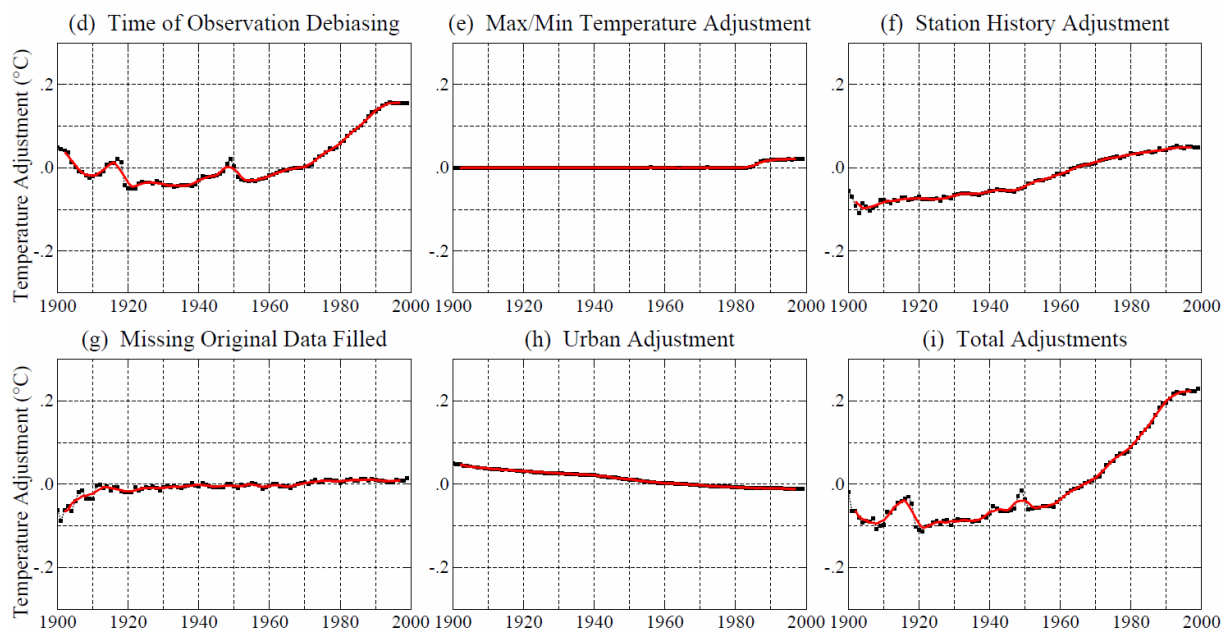
Figure 9. USHCN corrections (2001)
