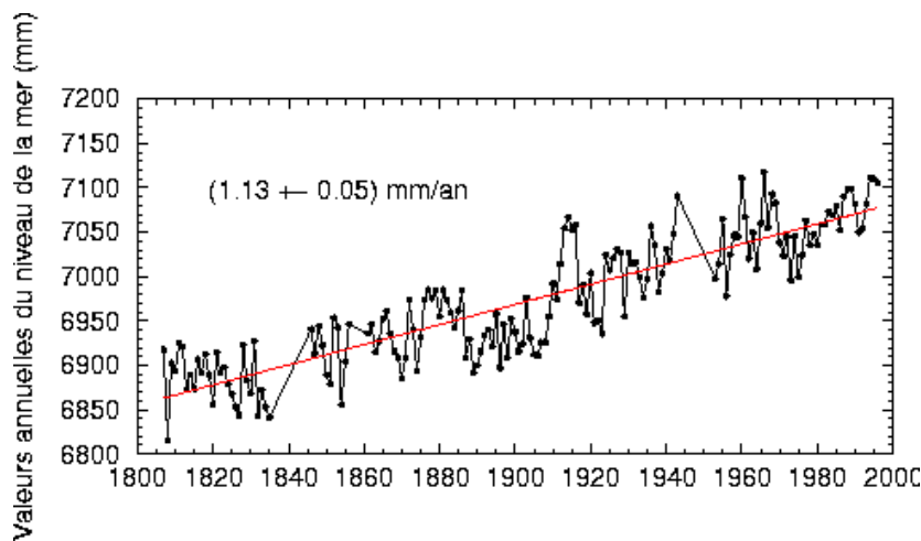
Figure 39: Changing sea levels over time at Brest [Desnoës]
