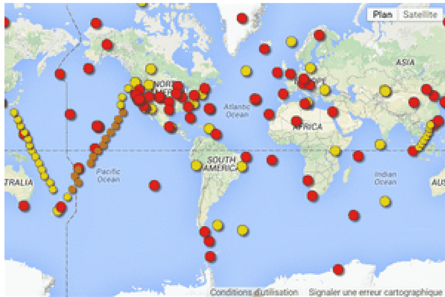
Figure 15. Location of laboratories taking flask samples. The red points are active sites, the yellow points are inactive sites, and the orange points are ship-based.
