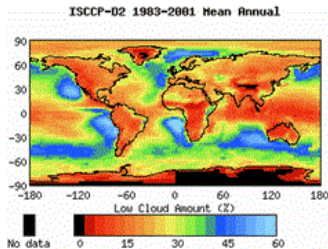
Figure 4: Low cloud cover (ISCCP)
