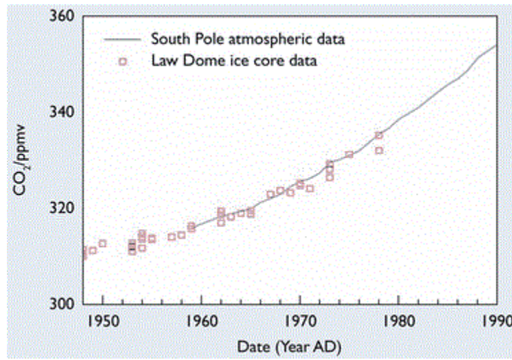
Figure 31. Direct measurements of CO 2 compared with ice-core measurements
