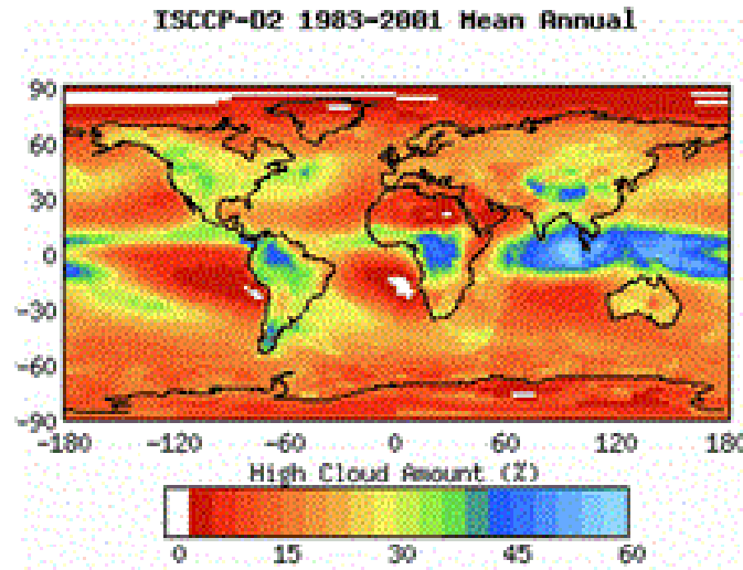
Figure 5: High cloud cover (ISCCP)
