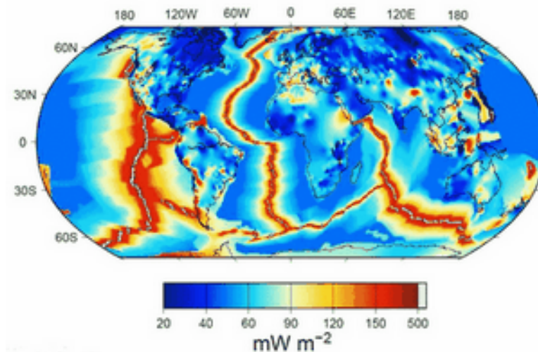
Figure 2: Map of global geothermal energy flow
