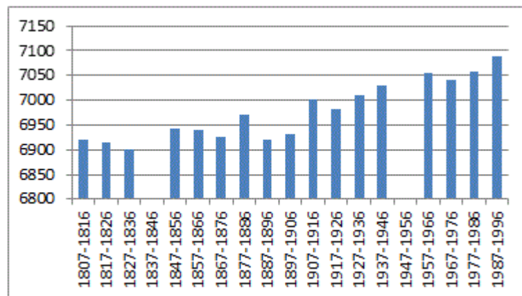
Figure 43: Average ocean level at Brest per decade
