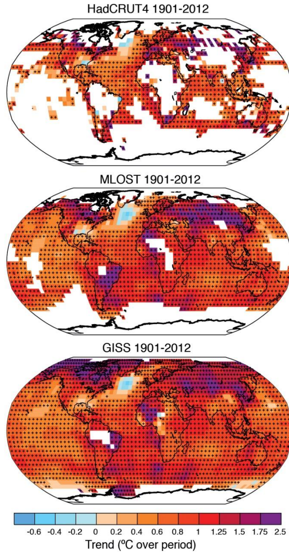
Figure 4: Change in surface temperature over 1901–2012 as determined by linear trend for three data sets [p. 39]
