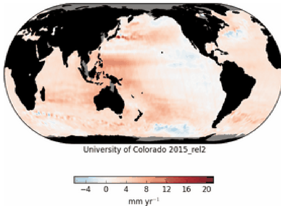
Figure 38: Regional sea level trends
