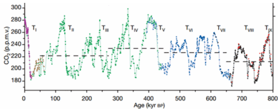
Figure 32. CO 2 measurements at Dome C (violet, blue and black), Taylor Dome (brown) and Vostok (green)
