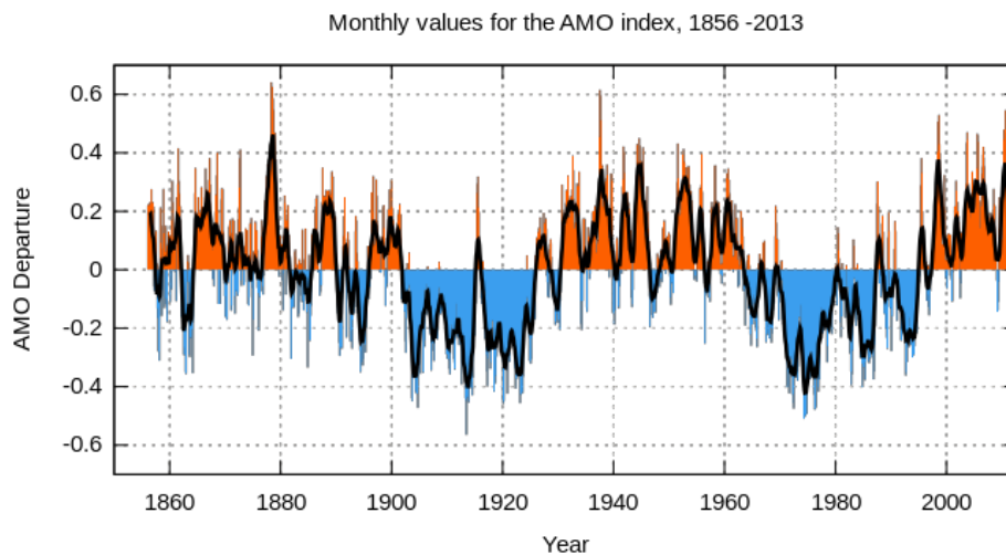
Figure 6: The Atlantic Multidecadal Oscillation
