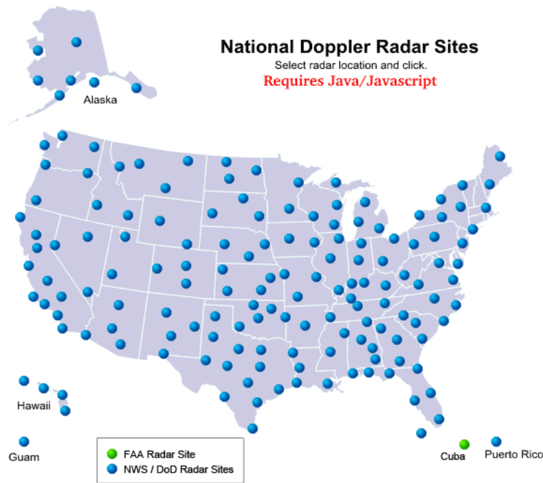
Figure 33. Distribution of radars in the US, according to the [NDRS]
