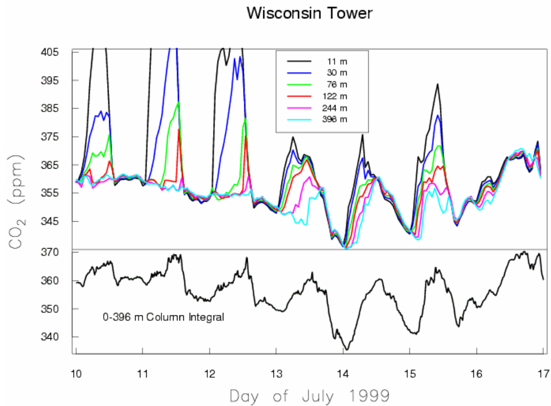
Figure 25. Measurements of CO 2 concentrations for a week in July 1999, Wisconsin Tower
