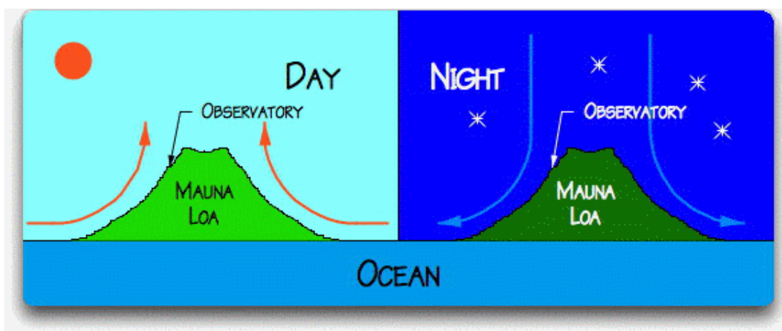
Figure 18. Air currents at Mauna Loa during the day and at night
