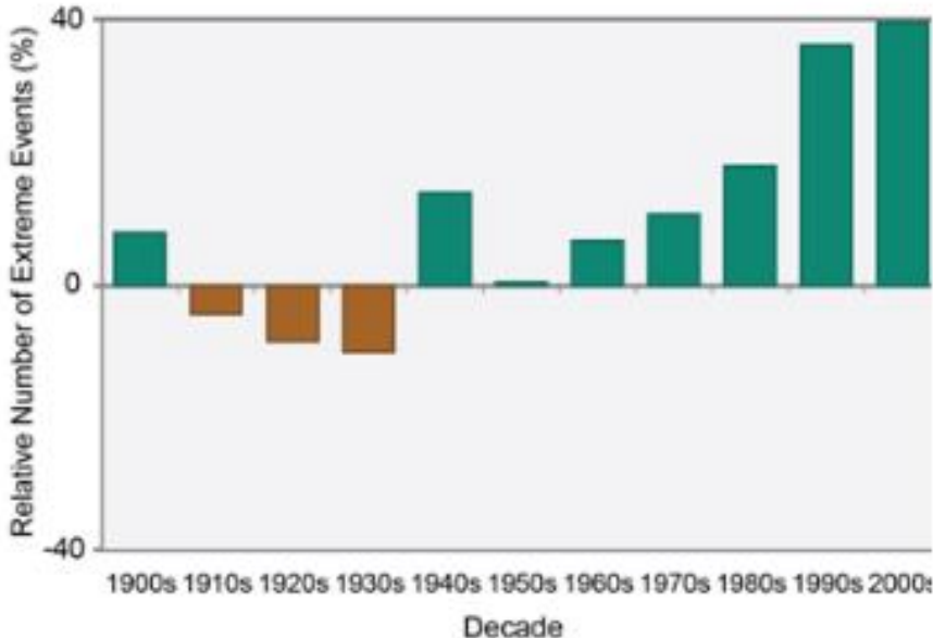
Observed U.S. Trend in Heavy Precipitation
